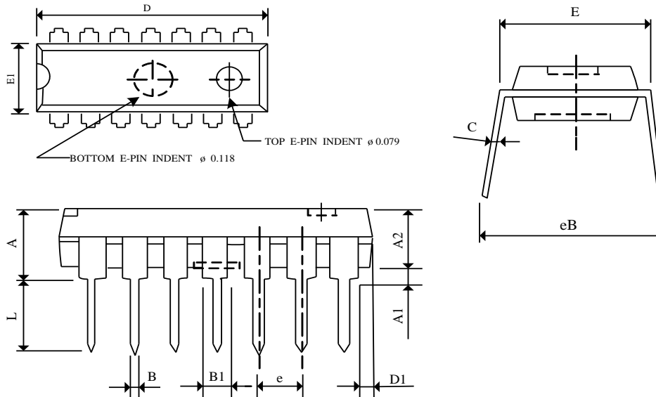
(a) 14 Pin DIP
