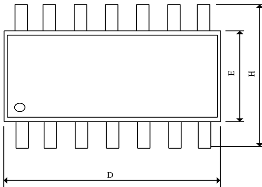
(b) 14 Pin SOP
